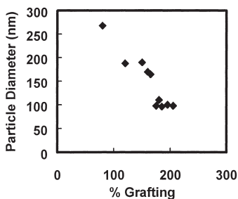
Fig 4. Correlation between particle diameter and percentage grafting, as well as TEM micrographs of casein-g-PMMA latexes
