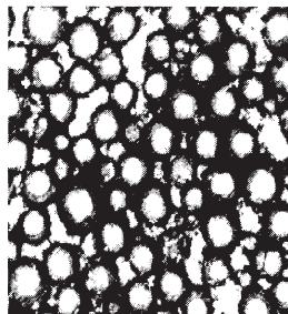
Fig 4. Correlation between particle diameter and percentage grafting, as well as TEM micrographs of casein-g-PMMA latexes
