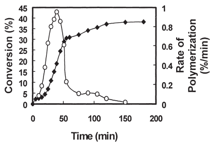
Fig 2. Conversion (◆) and rate of polymerization (○) vs reaction time ([MMA]=3%, [casein]=1%, [Cu^{2+}] = 7.5\text{ppm} , 70^{\circ}\text{C} )
